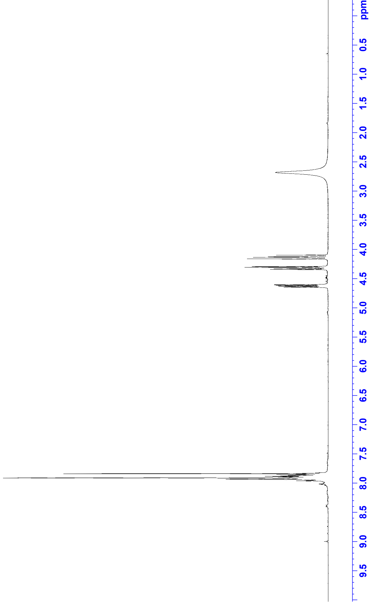
(S) - (+) -2-Phenylglycinol
