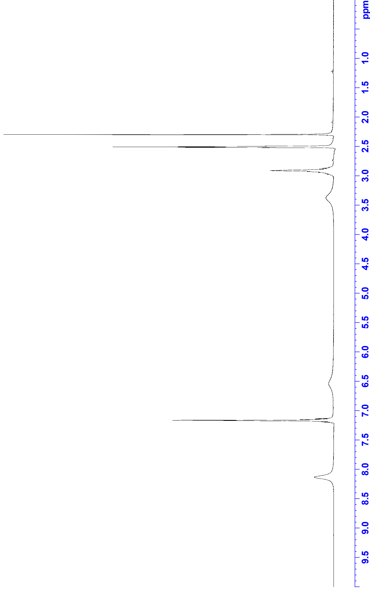
2-(2-methylphenyl)ethan-1-amine hydrochloride
